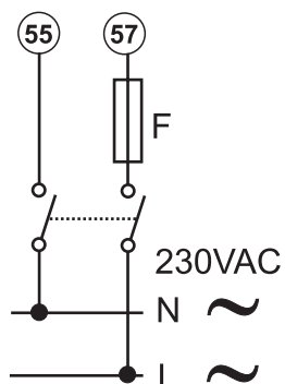
Fig. 21 D mulighed. F = 250\text{ V}, 50\text{ mA}
